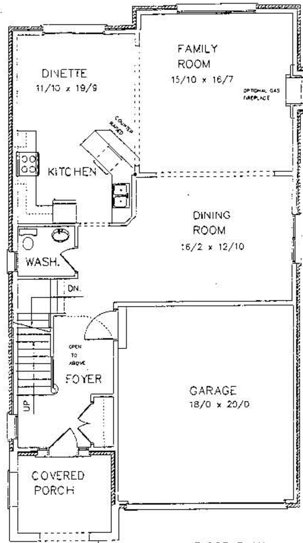
MAIN FLOOR PLAN
